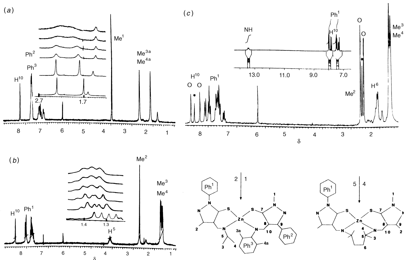
Fig. 5 The 200 MHz 1 H NMR spectra of complexes 1 (a), 2 (b) and 5 (c) in CDCl 2 CDCl 2 and of the pro-ligand H 2 L in CDCl 3 (inset) at 25 °C. Temperatures for the selected temperature-dependent spectra for complexes 1 and 2 are (from bottom to top) 25, 80, 105, 115, 125 and 130 °C (same scale)
