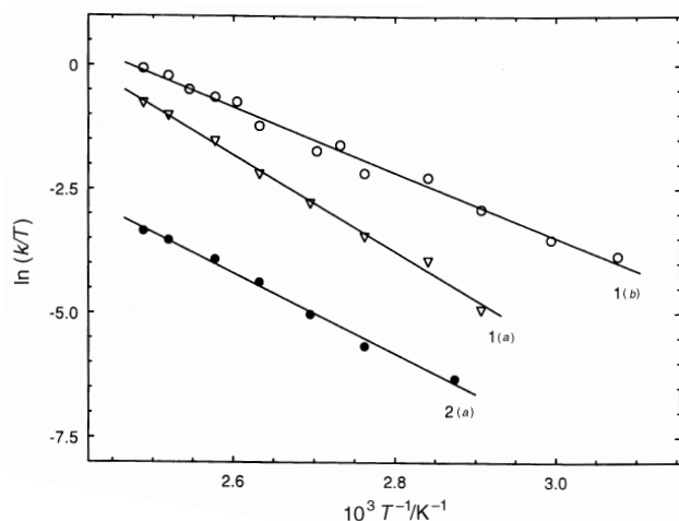
Fig. 7 Eyring plots (a) for complexes 1 and 2 in CDCl 2 CDCl 2 and (b) for 1 in C 6 D 5 NO 2
