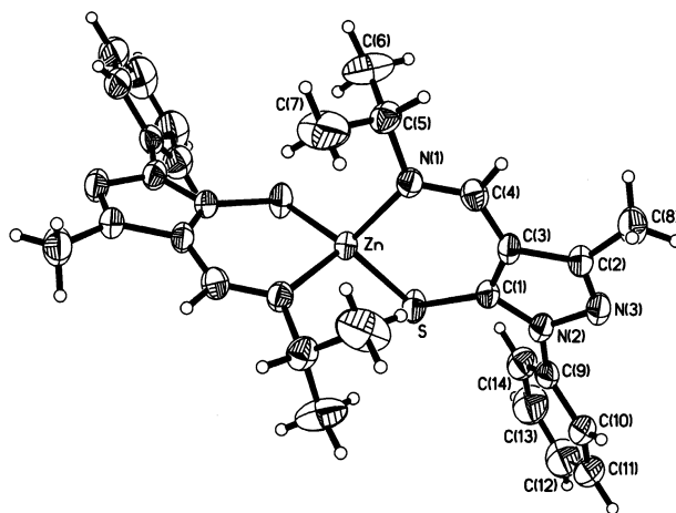
Fig. 3 Molecular structure of complex 2 , with 50% probability thermal ellipsoids for non-hydrogen atoms
