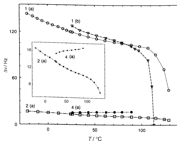
Fig. 6 Plots of Δν vs. T for complexes 1 , 2 and 4 in (a) CDCl 2 CDCl 2 and (b) C 6 D 5 NO 2
